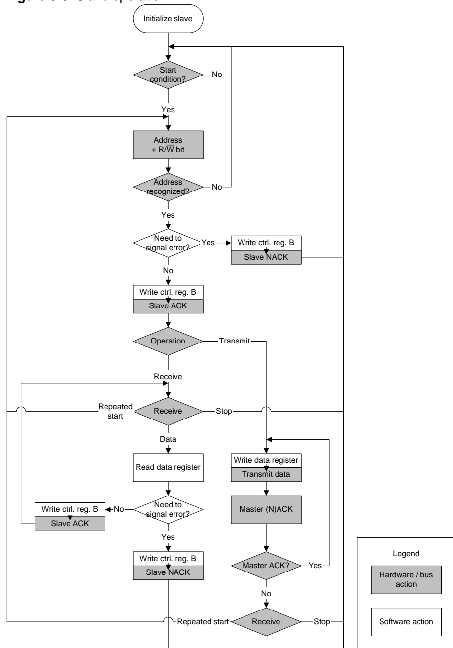
Figure 3-3. Slave operation.
