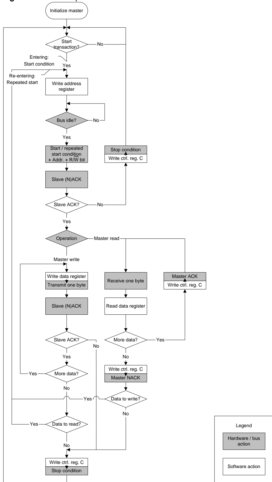
Figure 3-2. Master operation.
